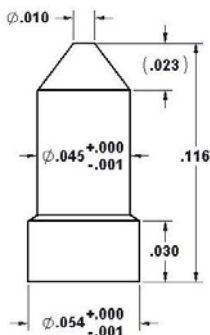
92-30099 Ø.054" Base/Ø.010" Flat Tip
