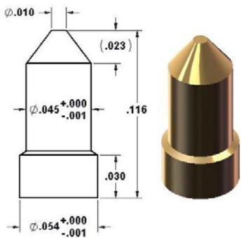
92-30099 \varnothing.054 " Base/ \varnothing.010 " Flat Tip
