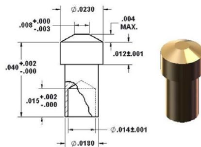
92-30750 \varnothing.0180 " Base/ \varnothing.008 " Flat Tip
