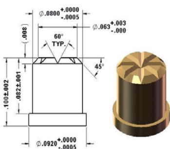
92-30083 \varnothing.0920 " Base/ \varnothing.063 " Multi-Point
