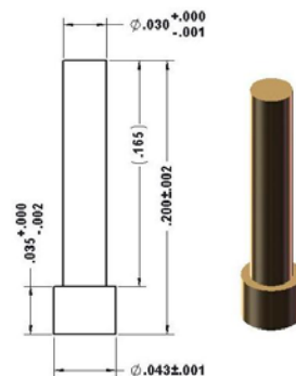
92-30667 Ø.043" Base/Ø.030" Flat Tip
