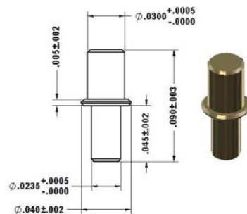
92-3717 \varnothing.0235 " Base/ \varnothing.0300 " Flat Tip
