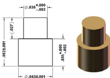
92-30676-1 \varnothing.043 " Base/ \varnothing.030 " Flat Tip
