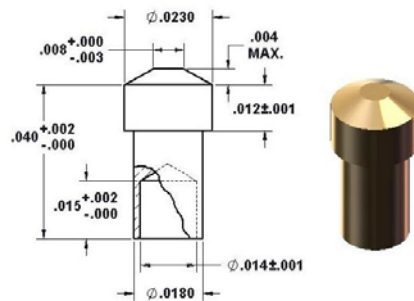
92-30750 Ø.0180" Base/Ø.008" Flat Tip
