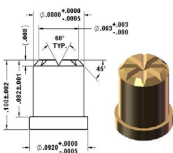
92-30083 Ø.0920" Base/Ø.063" Multi-Point
