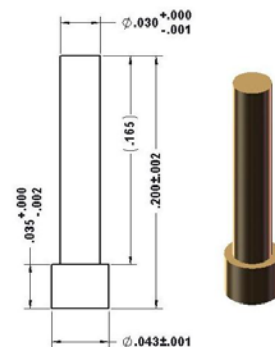
92-30667 \varnothing.043 " Base/ \varnothing.030 " Flat Tip
