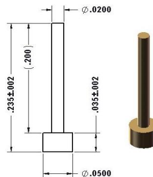
92-30640 Ø.050" Base/Ø.020" Contact Pin
