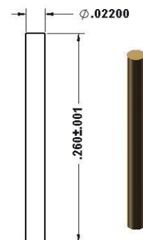
92-30724 Ø.0220" Cylindrical
