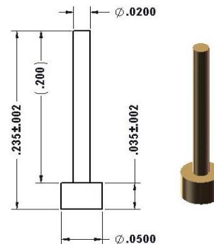
92-30640 Ø.050" Base/Ø.020" Contact Pin
