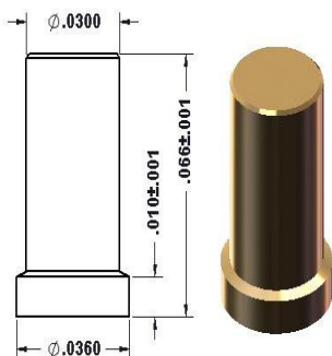
92-30719 Ø.0360" Base/Ø.0300" Flat Tip
