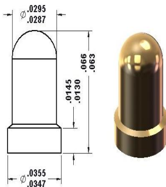
92-30080 Ø.0355" Base/Ø.0295" Spherical Tip
