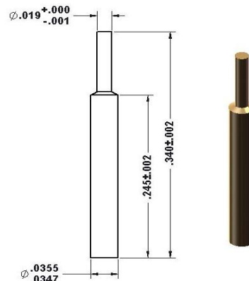
92-30032-1 Ø.0347" Base/Ø.019" Flat Tip
