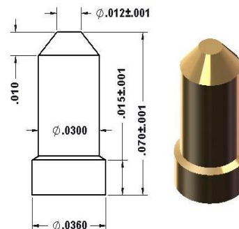
92-30090 Ø.0360" Base/Ø.012" Flat Tip
