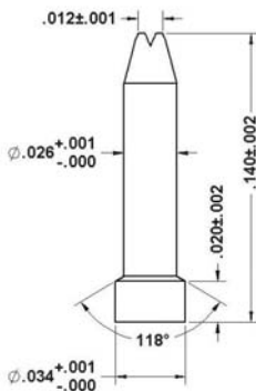
92-30053 Ø.034" Base/Ø.026" Flat Tip
