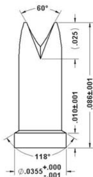
92-30703 Ø.0355" Base/Ø.0295" Crown Tip
