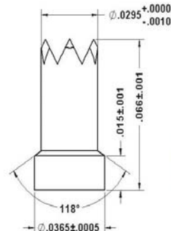
92-30048-1 Ø.0365" Base/Ø.0295" Serrated Tip
