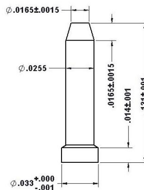
92-30027-1 Ø.0330" Base/Ø.0165" Flat Tip
