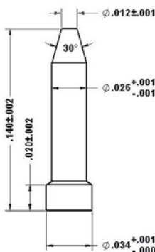
92-30060 Ø.034" Base/Ø.012" Flat Tip
