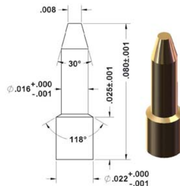
92-30037 Ø.022" Base/Ø.008" Flat Tip
