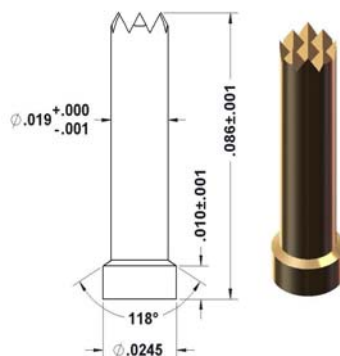
92-30711 Ø.0245" Base/Ø.019" Serrated Tip
