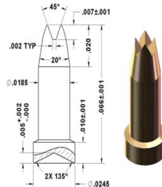
92-30715-2 Ø.0245" Base/Ø.0185" Crown Tip
