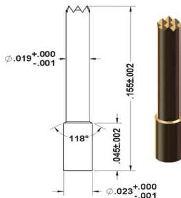
92-30259 Ø.023" Base/Ø.019" Serrated Tip
