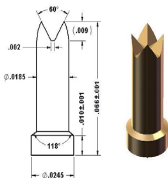
92-30045 Ø.0245" Base/Ø.0185" Crown Tip
