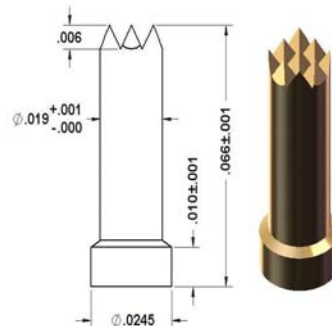
92-30028-5 Ø.0245" Base/Ø.019" Serrated Tip
