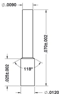
92-30051 Ø.012" Base/Ø.009" Flat Tip
