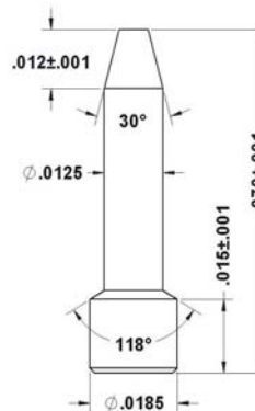
92-30753-1 Ø.0185" Base/Ø.006" Flat Tip
