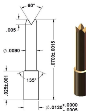
92-30723 Ø.012" Base/Ø.009" Crown Tip
