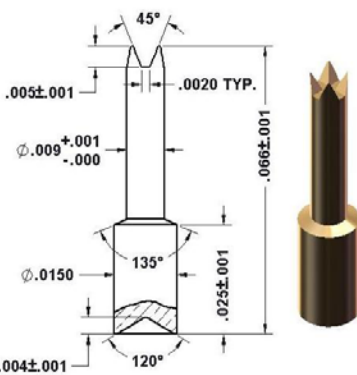
92-30730 Ø.015" Base/Ø.009" Crown Tip
