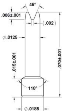
92-30759 Ø.0185" Base/Ø.0125" Crown Tip
