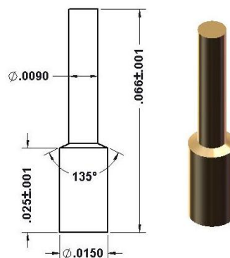
92-30741 Ø.015" Base/Ø.009" Flat Tip
