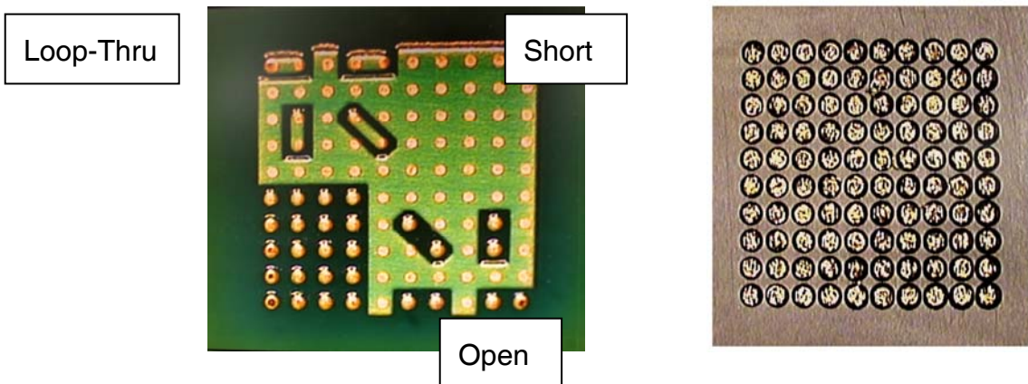
Figure 1: Surrogate Package (left) and a typical 10 x 10 Socket / Interconnect array (right)
