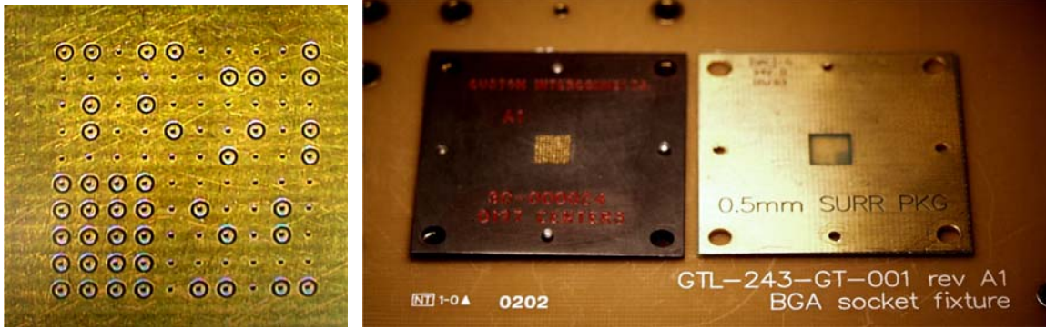
Figure 2 : Fixture showing Probe Side (left) and Socket / Interconnect Side with sample and Surrogate (right)
